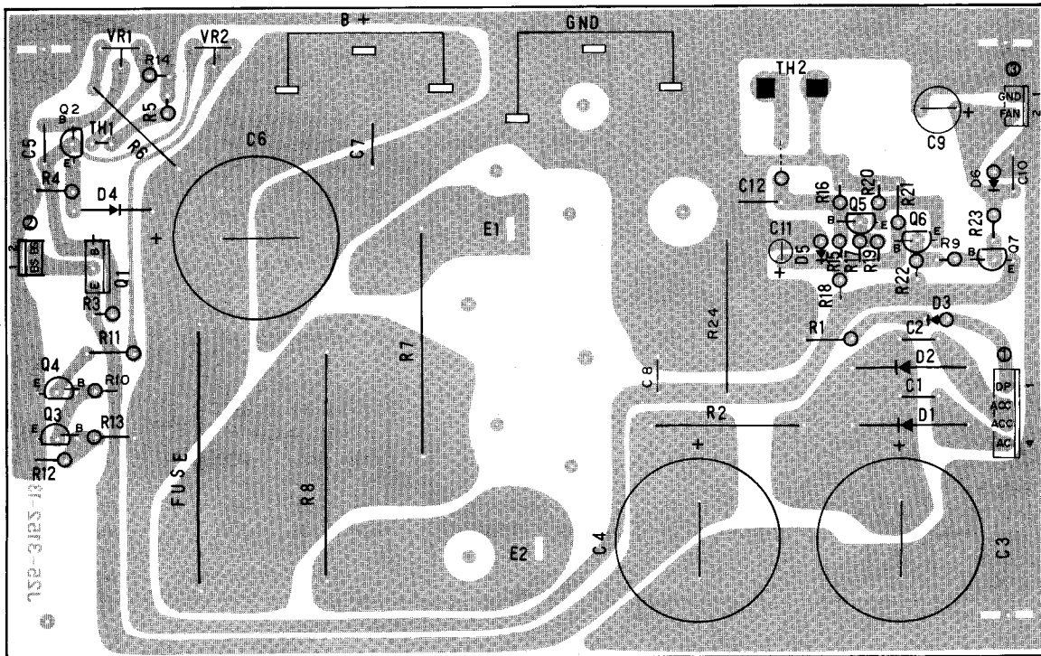
AVR UNIT (X43-1440-00) Component side view
